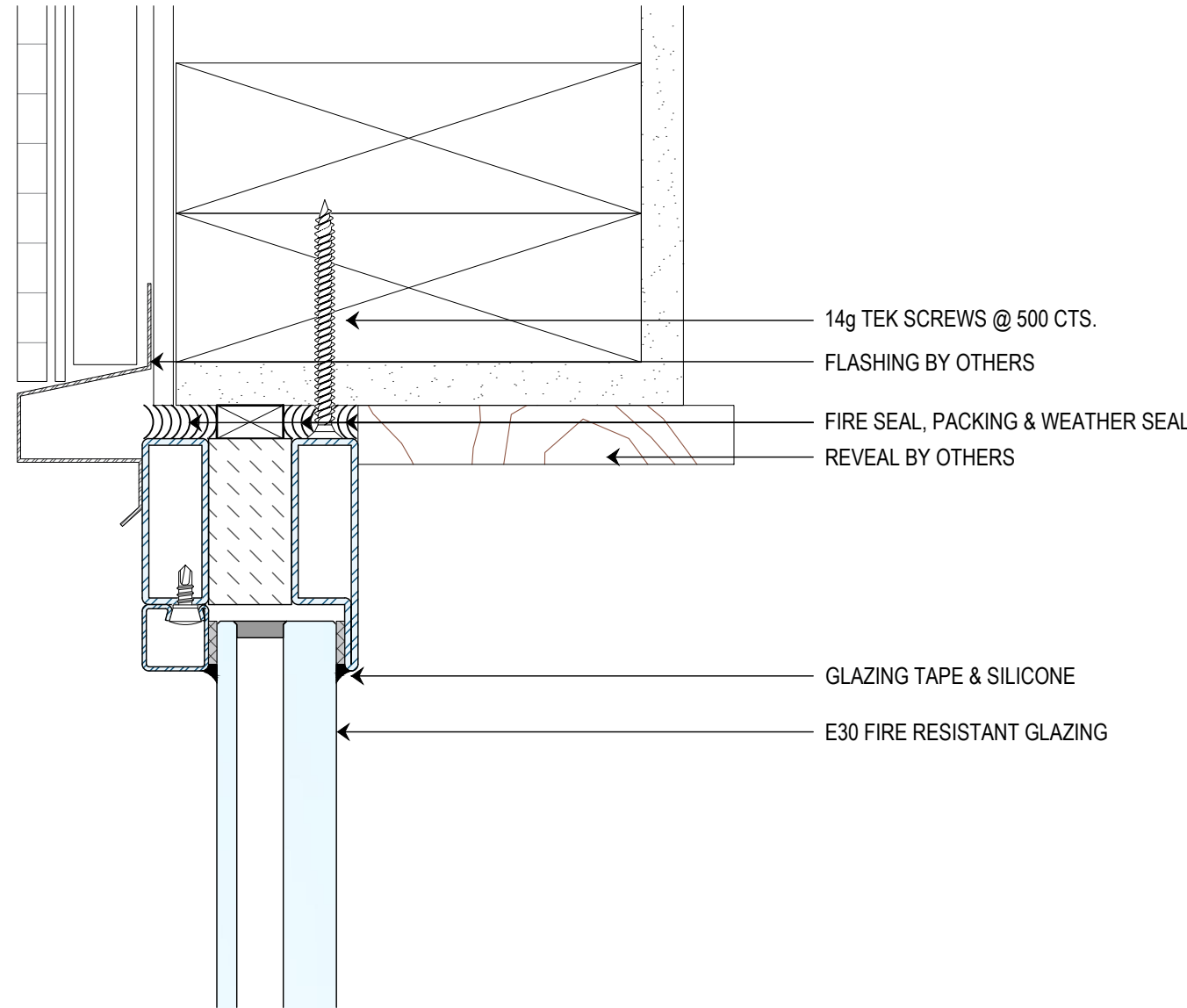
3 FIXED WINDOW HEAD DETAIL INTO STUD SCALE 1:2 @ A2
