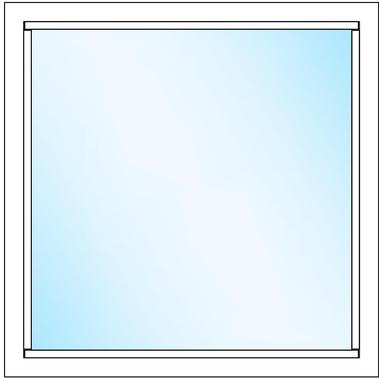
1 VIEW FROM OUTSIDE VISIONEERING WINDOW -/30/30 SCALE 1:10 @ A2
