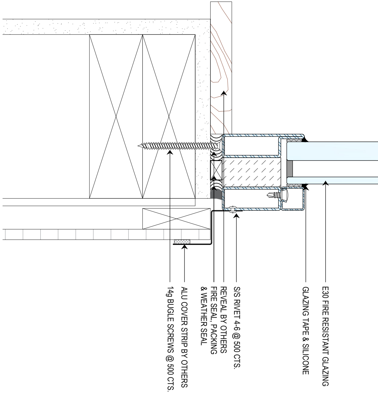
2 FIXED WINDOW JAMB DETAIL INTO STUD SCALE 1:2 @ A2
