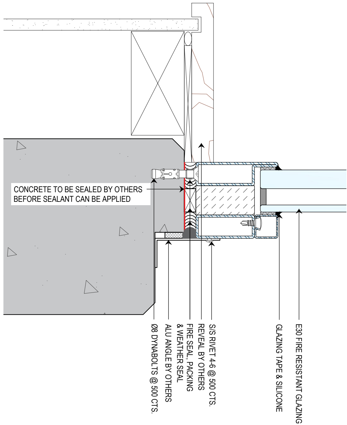
1 FIXED WINDOW JAMB DETAIL INTO PC SCALE 1:2 @ A2
