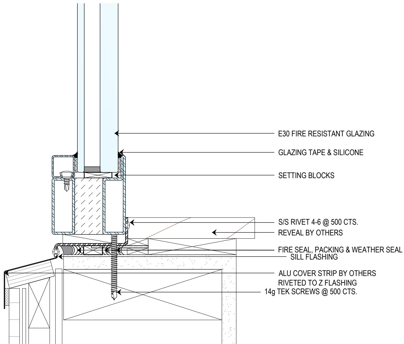
4 FIXED WINDOW SILL DETAIL INTO STUD SCALE 1:2 @ A2
