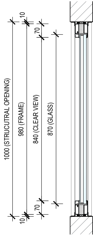
A SIDE ELEVATION SECTION SCALE 1:10 @ A2
