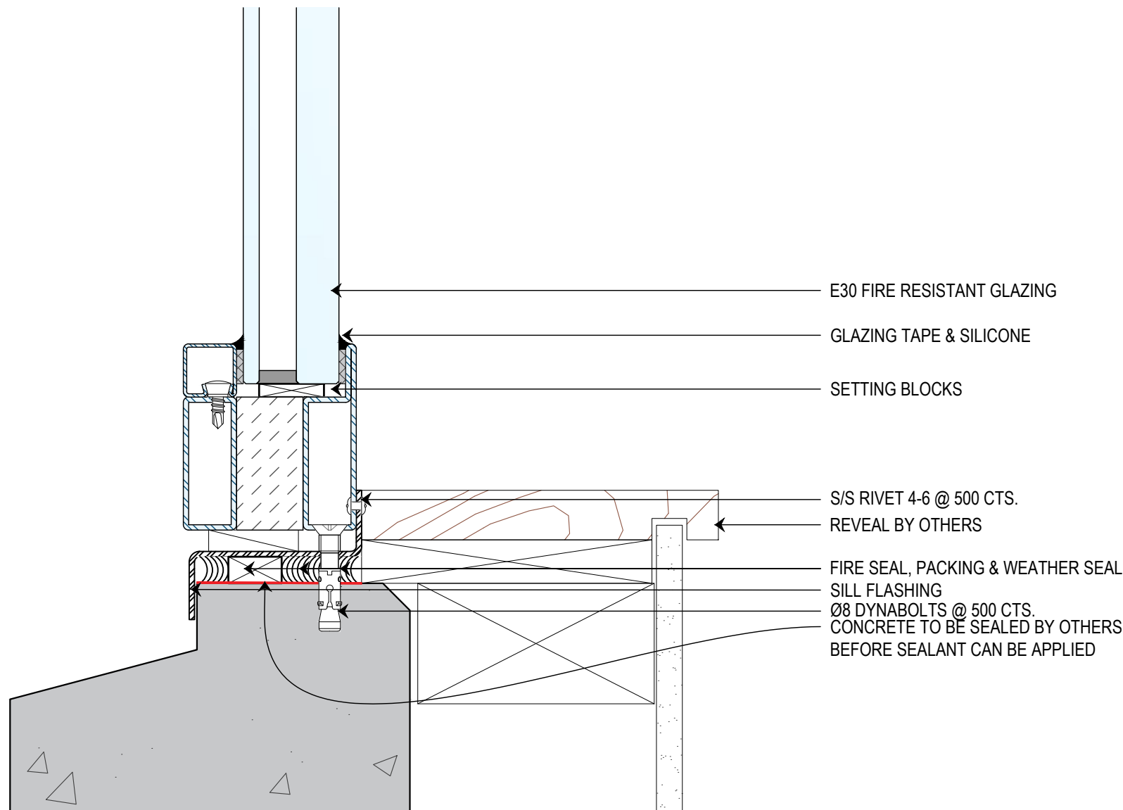
2 FIXED WINDOW SILL DETAIL INTO PC SCALE 1:2 @ A2
